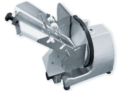
Steeply inclined carriage with guide rail and guide ribs for non-stick effect
